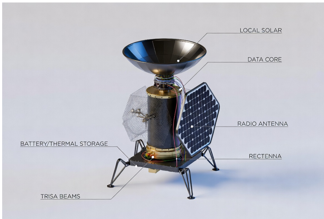
Figure 1. Flame Hearth — unified energy storage, rectenna, local solar, data core, and mesh antenna. Small. Discrete. Replicable.
